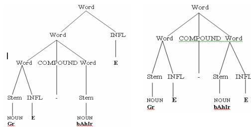
Figure 7: Two parse trees for the word “GrE-bAhIrE” (ঘরে-বাহিরে)
