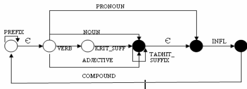
Figure 5: FSM for compound word (version 2)
