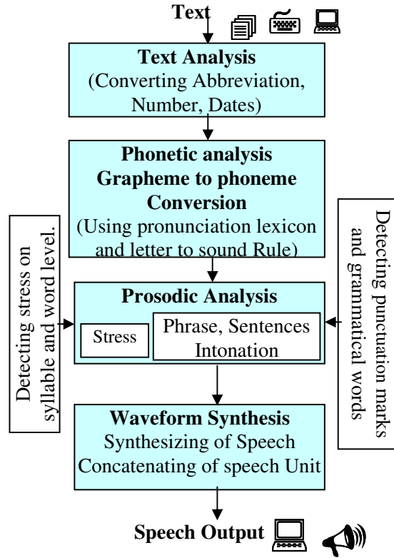
Figure 1: Architecture of TTS
