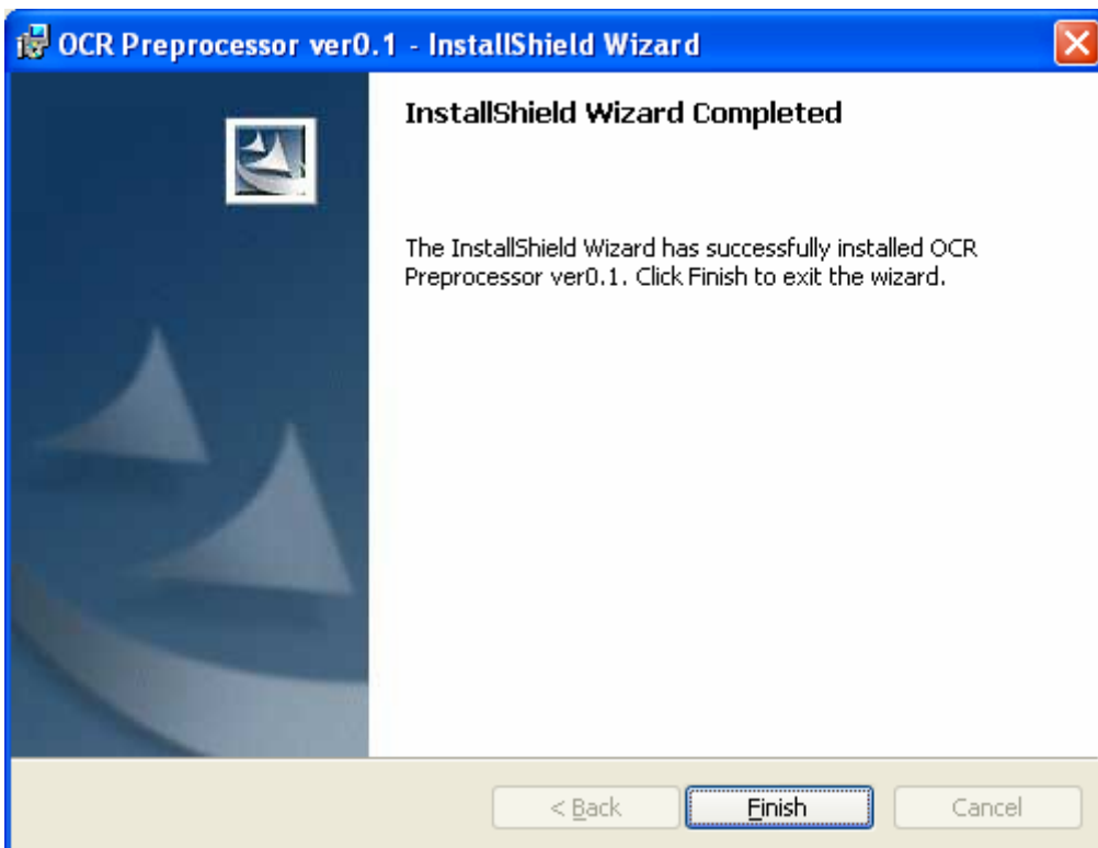
Figure 3.4: Setup complete
