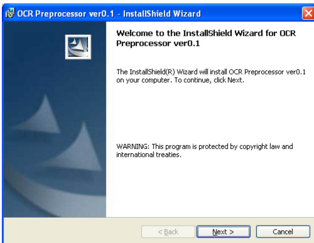
Figure 3.1: Welcome window
