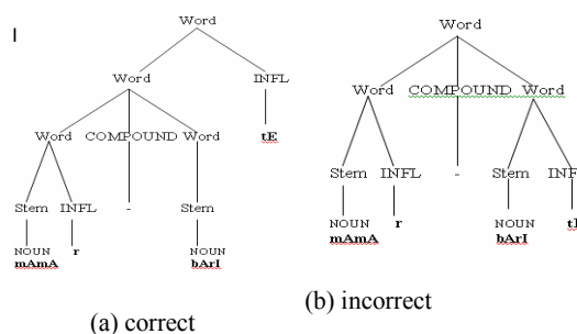
Figure 6: Two parse trees for the word “mAmAr-bArItE” (মামার-বাড়িতে)
