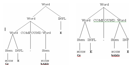
Figure 7: Two parse trees for the word “GrE-bAhrE” (ঘরে-বাহিরে)
