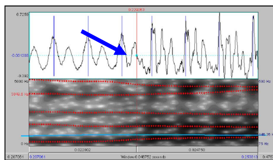
Figure 2: Splitting at the zero crossing position
