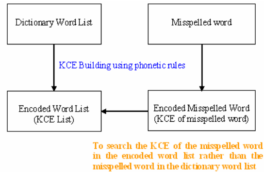
Figure 1: KCE building using phonetic rules
